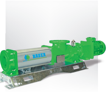
HELIX DRIVE Eccentric screw pump
